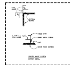
LEAD ANGLE SYSTEM CORNER DETAIL
