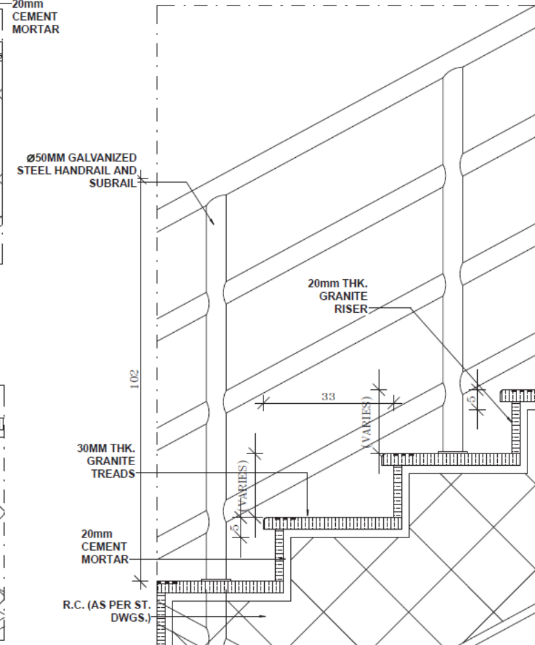
STEEL HANDRAIL DETAIL
