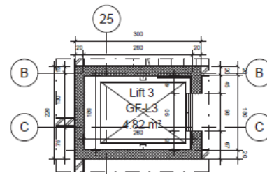
6 AR-015 LIFT 3 GF DETAIL PLAN 1 : 50
