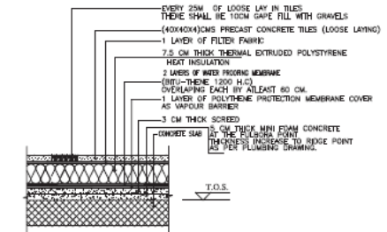
TYPICAL ROOF FINISHING DETAIL
