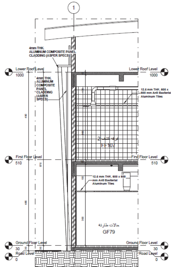
3 WALL SECTION C 1:50
