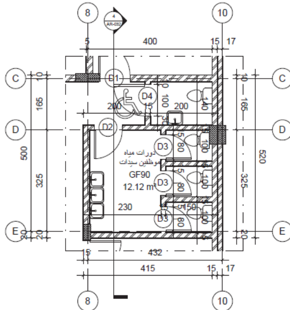
1 TOILET DETAILS-GF90 1:50 AR-032
