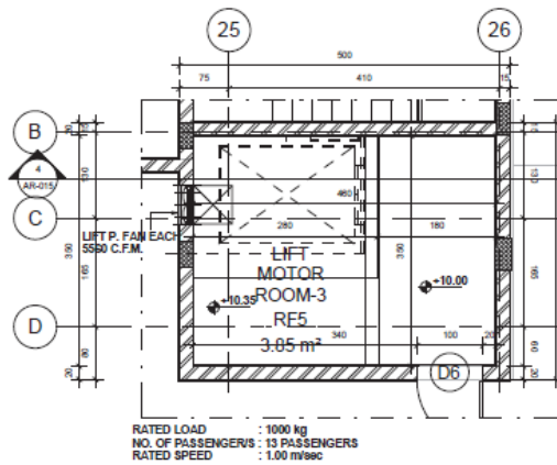
5 AR-015 LIFT MOTOR ROOM 3 1 : 50
