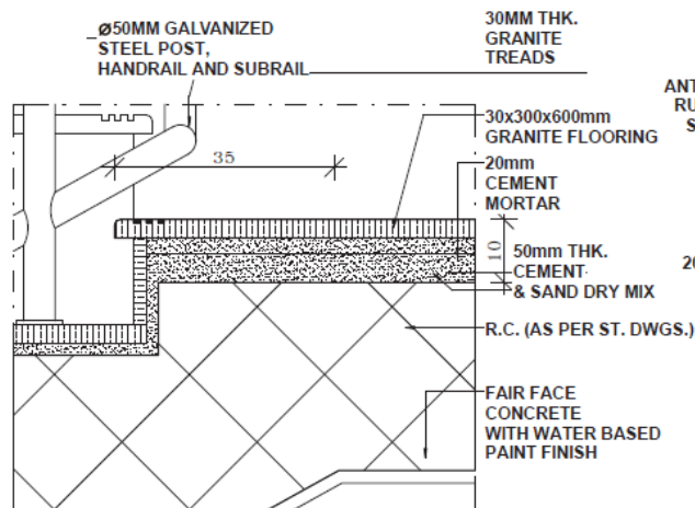
STAIRHEAD DETAIL
