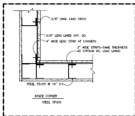
INSIDE CORNER STEEL STUDS
