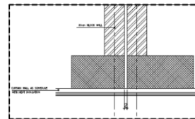
GROUND FLOOR EXPANSION JOINT DETAIL
