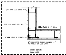
OUTSIDE CORNER STEEL STUDS
