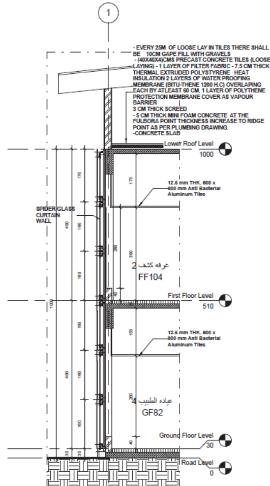
2 WALL SECTION B 1:50
