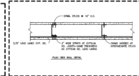
WALL DETAIL
