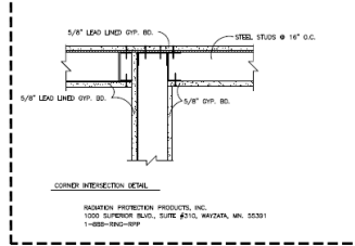
CORNER INTERSECTION DETAIL STEEL STUDS
