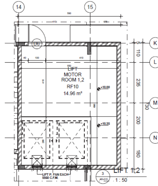
2 AR-015 LIFT MOTOR ROOM 1,2 1 : 50
