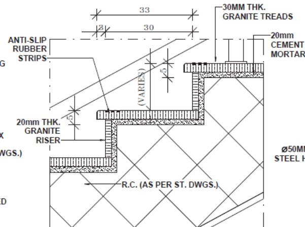
RISER & TREAD DETAIL
