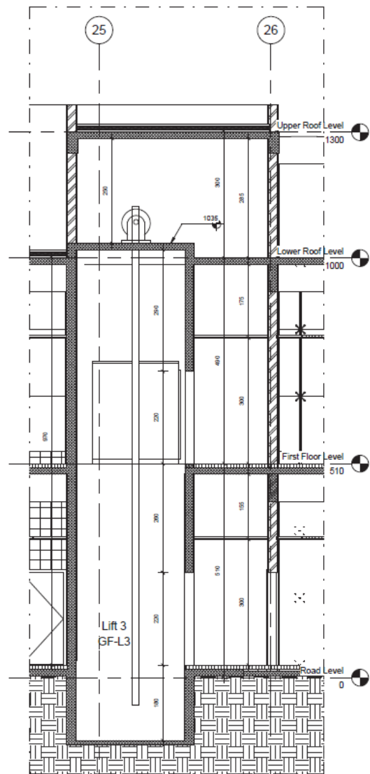
4 AR-015 LIFT 3 1 : 50
