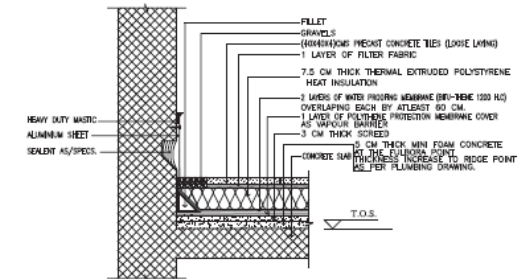
TYPICAL ROOF FINISHES WITH PARAPET WALL
