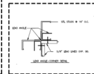
LEAD ANGLE - CORNER DETAIL
