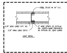
JOINT DETAIL
