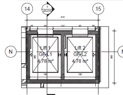
1 AR-015 LIFT 1,2 GF DETAIL PLAN 1 : 50
