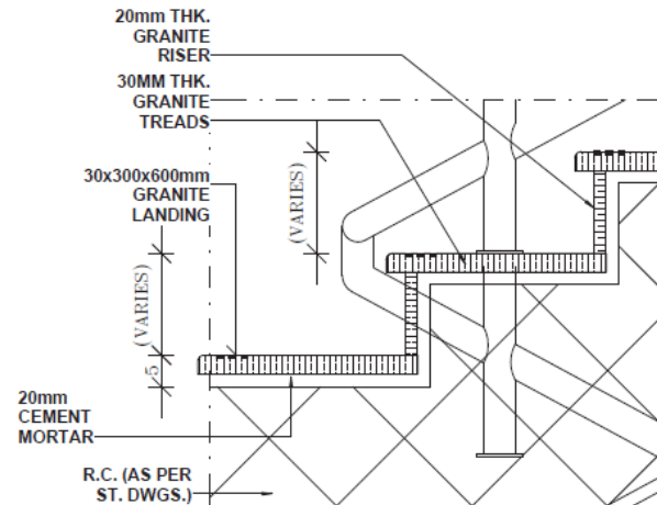
LANDING DETAIL
